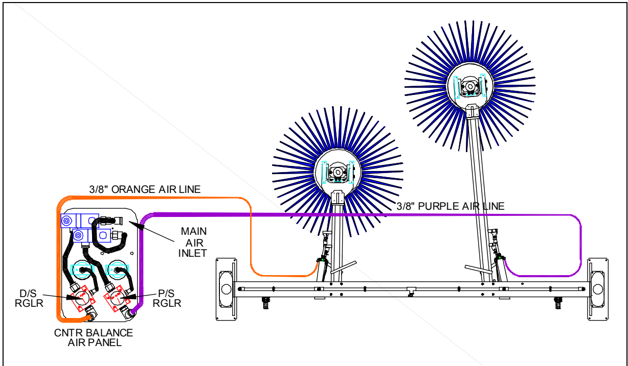
Pic #3 Pull Air Lines
