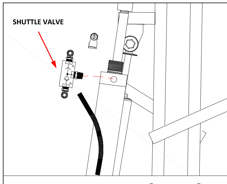
Pic #2 Install Shuttle Valves Assembly
